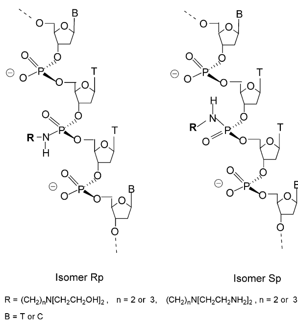
Figure 1. Structures of the modified internucleotide linkages.
