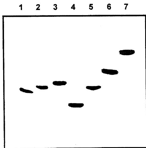
Figure 4. Denaturing polyacrylamide (20%) gel electrophoresis of modified and unmodified 17-mers oligo-2'-deoxyribonucleotides stained with methylene blue: lane 1: TFO 7 , lane 2: TFO 8 , lane 3: TFO 9 , lane 4: TFO 13 , lane 5: TFO 10 , lane 6: TFO 11 , lane 7: TFO 12 .
