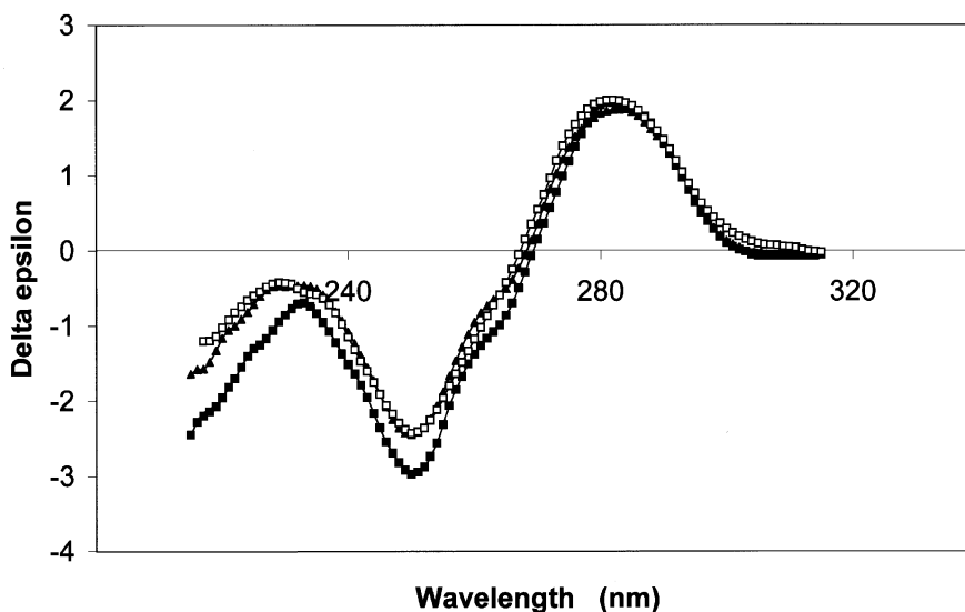
Figure 6. Cd spectra of the triplexes containing the modified oligonucleotide 9 (▲), 12 (■), and unmodified oligonucleotide 13 (□) at pH 5.5 and 20 °C.
