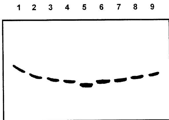
Figure 3. Denaturing polyacrylamide (20%) gel electrophoresis of modified and unmodified 22-mer oligo-2'-deoxyribonucleotides stained with methylene blue: lane 1: TFO 2a , lane 2: TFO 2b , lane 3: TFO 3a , lane 4: TFO 3b , lane 5: TFO 6 , lane 6: TFO 4a , lane 7: TFO 4b , lane 8: TFO 5a , lane 9: TFO 5b .
