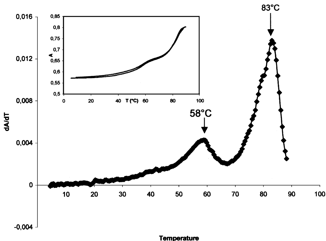
Figure 5. UV-melting profile for the triplex containing oligonucleotide 12 at pH 5.5. The ordinate shows the first derivative of the melting curve dA/dT , while the insert shows the melting curve.
