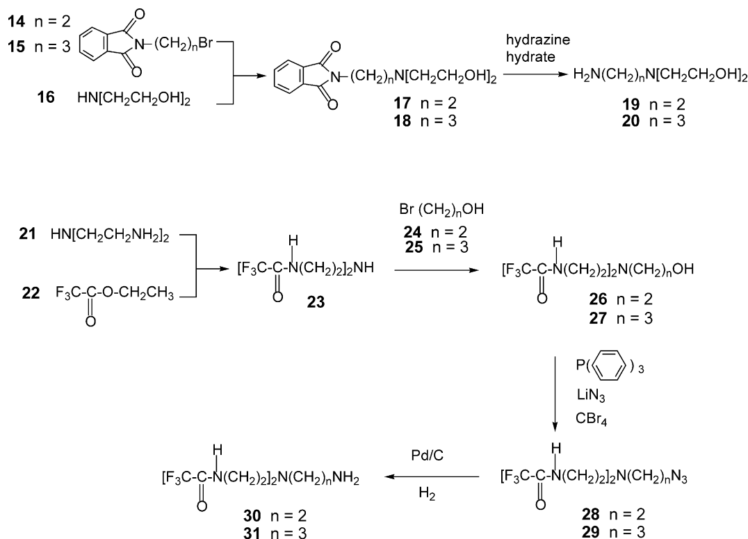
Scheme 1. Synthesis of substituent groups 19 , 20 , 30 and 31 used for the internucleotidic modifications.
