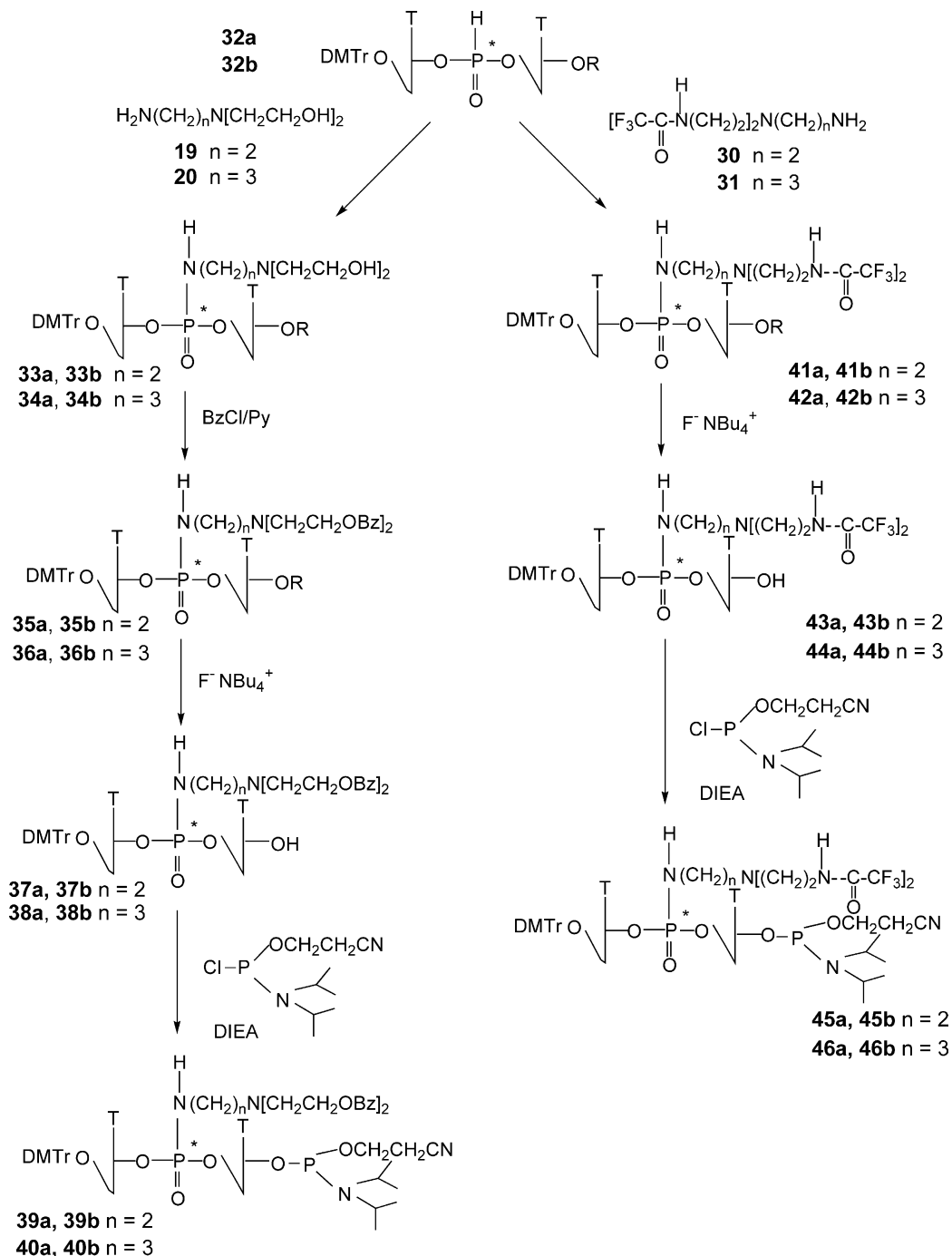
Scheme 2. Synthesis of modified dinucleoside-3'-phosphoramidites 39a–40b and 45a–46b. R = tert -butyldimethylsilyl, Bz = benzoyl.
