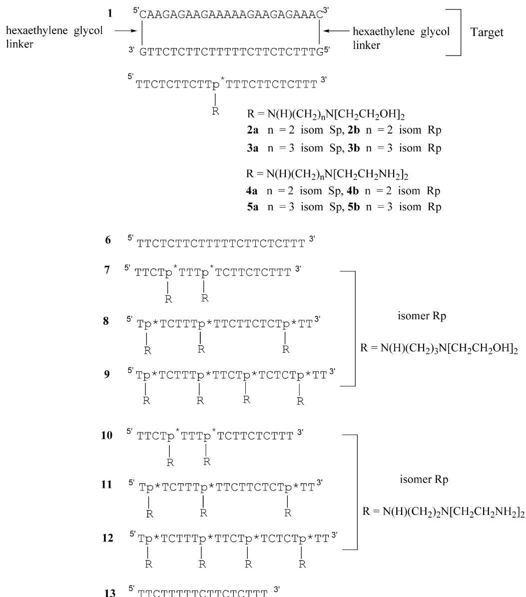
Figure 2. Chemical structures of triple-helical complexes. The sequences of the circularized 24-bp long double-stranded target containing the 22-bp long oligopyrimidine-oligopurine sequence and the third strands are depicted.
